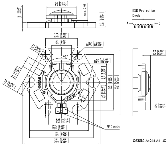
Dimensions in mm (inch). / Maße in mm (inch).
